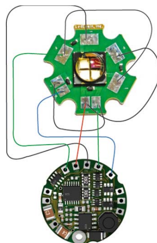
Sample wiring schematic of L-Dot Pico with LedEngine 10W RGB
